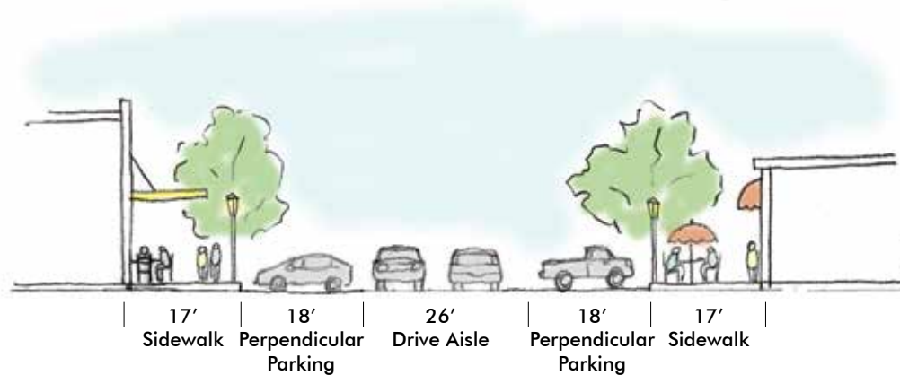
SECTION VIEW
