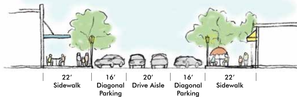
SECTION VIEW
