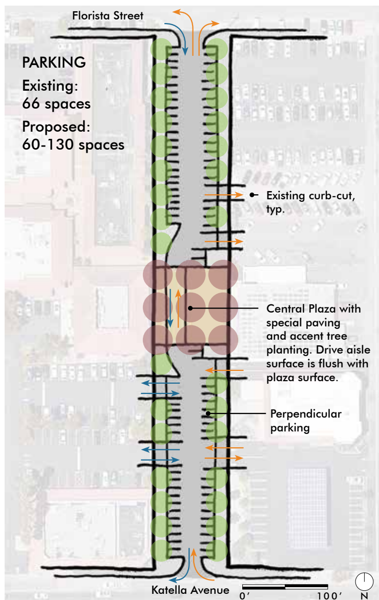
PLAN VIEW
